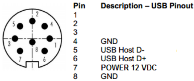
Figure 5. Pin-out for GXX-4GE
