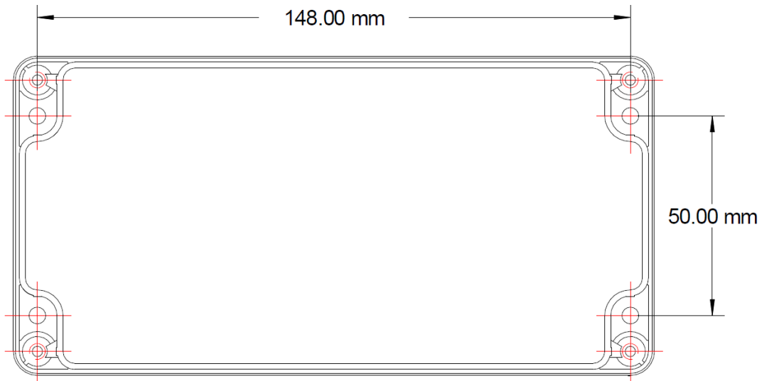
Figure 6. Drawing for mounting of GXX-4GE (units: mm)
