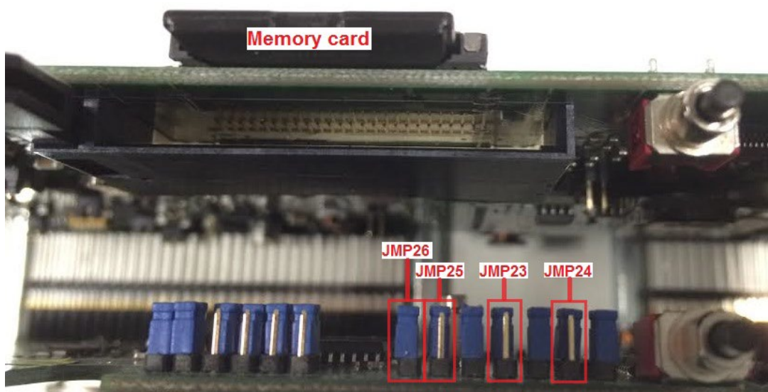
Figure 3. Standard jumper settings on the GMSplus connector board for GXX-4GE modem
