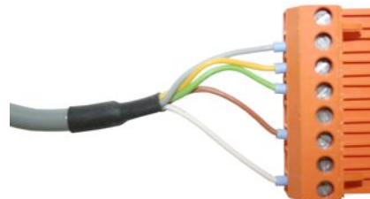
Figure 5. Connector wiring GXR-GPS-485
