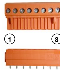
Figure 3. Connector pin out GXR-GPS-485
