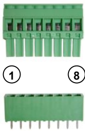
Figure 2. Connector pin out GXR-GPS
