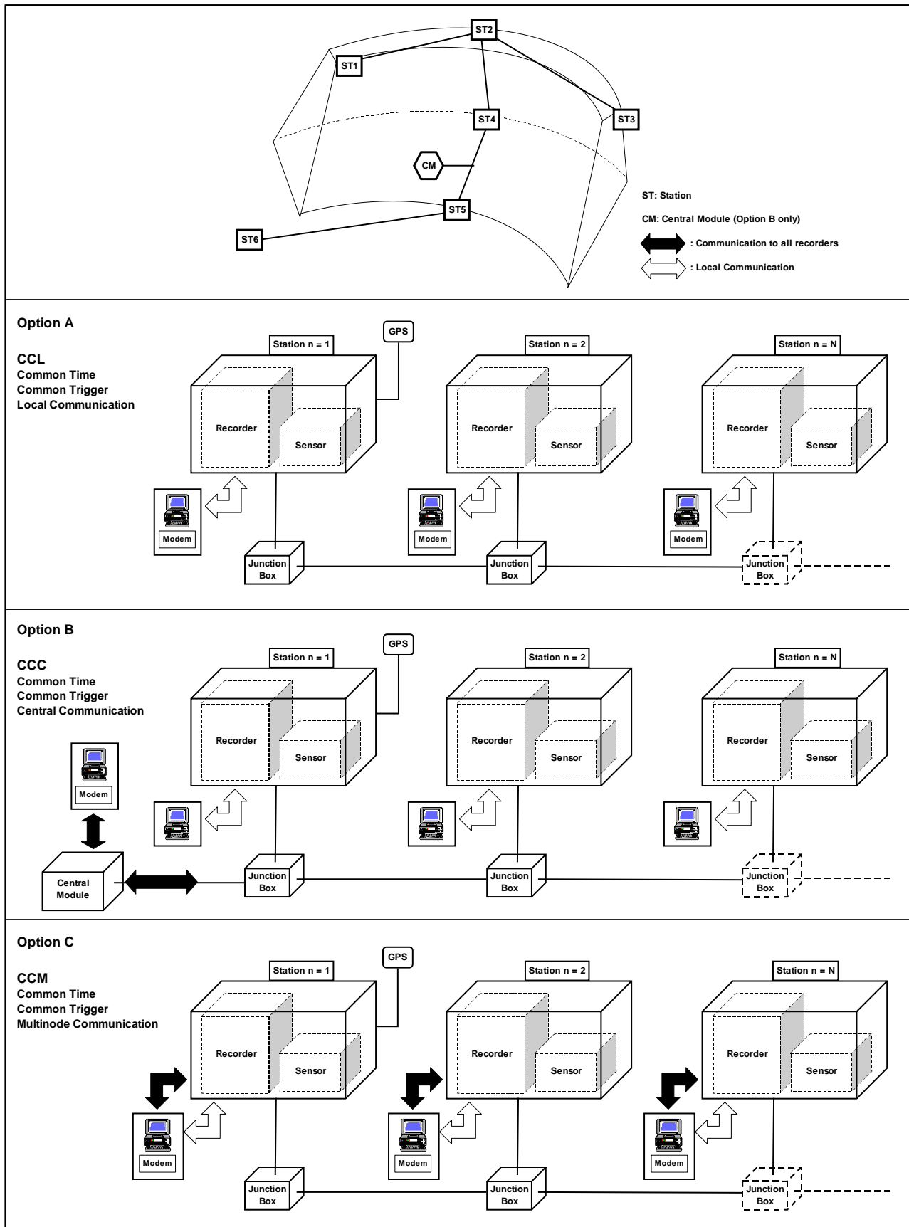
Figure 1. Topology of the Interconnected Recording Network Options
